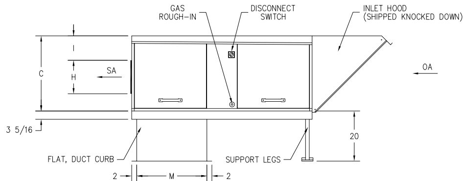
CONTROL SIDE VIEW
