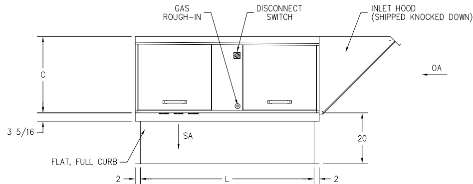
CONTROL SIDE VIEW
