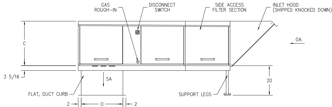
CONTROL SIDE VIEW
