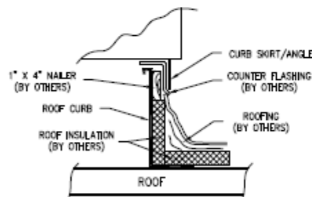
MOUNTING DETAIL FOR ROOF CURB
