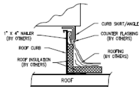
MOUNTING DETAIL FOR ROOF CURB
