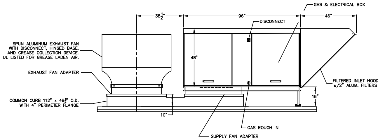
ELEVATION VIEW
