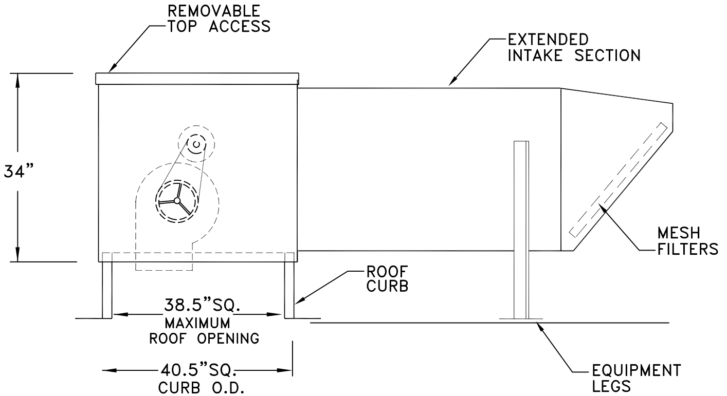
SECTION VIEW
