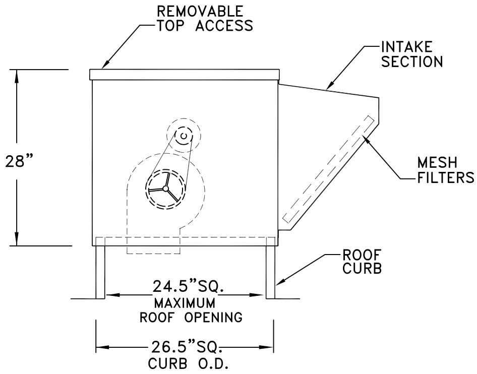
SECTION VIEW
