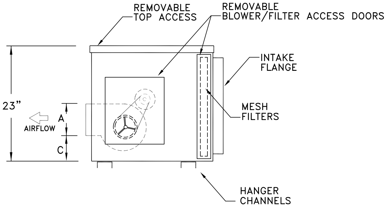
SECTION VIEW
