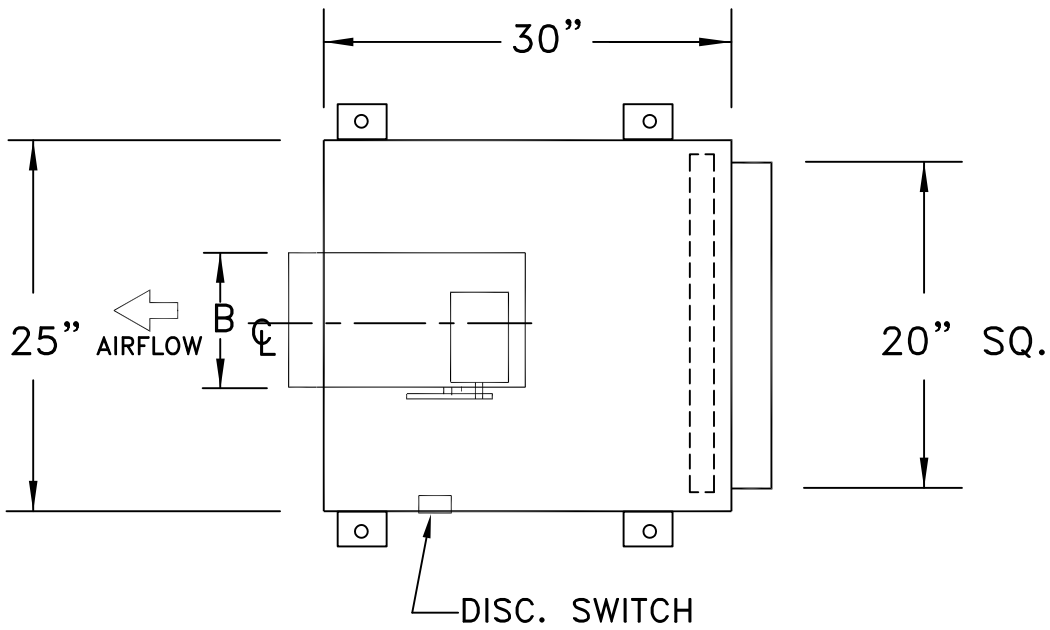
PLAN VIEW
