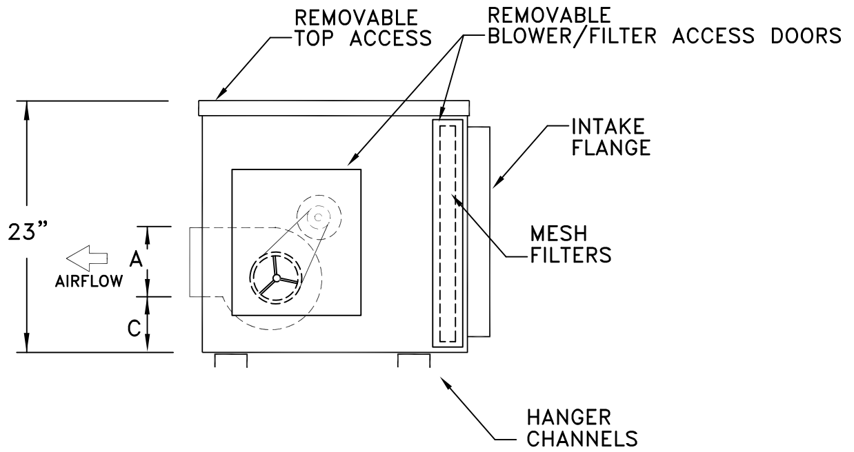
SECTION VIEW
