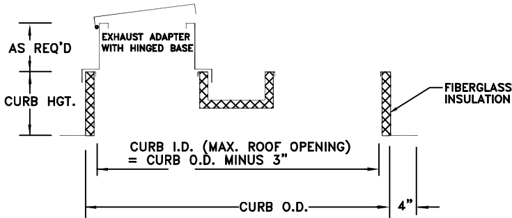
MODEL RCC
