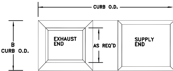
MODEL RCC
