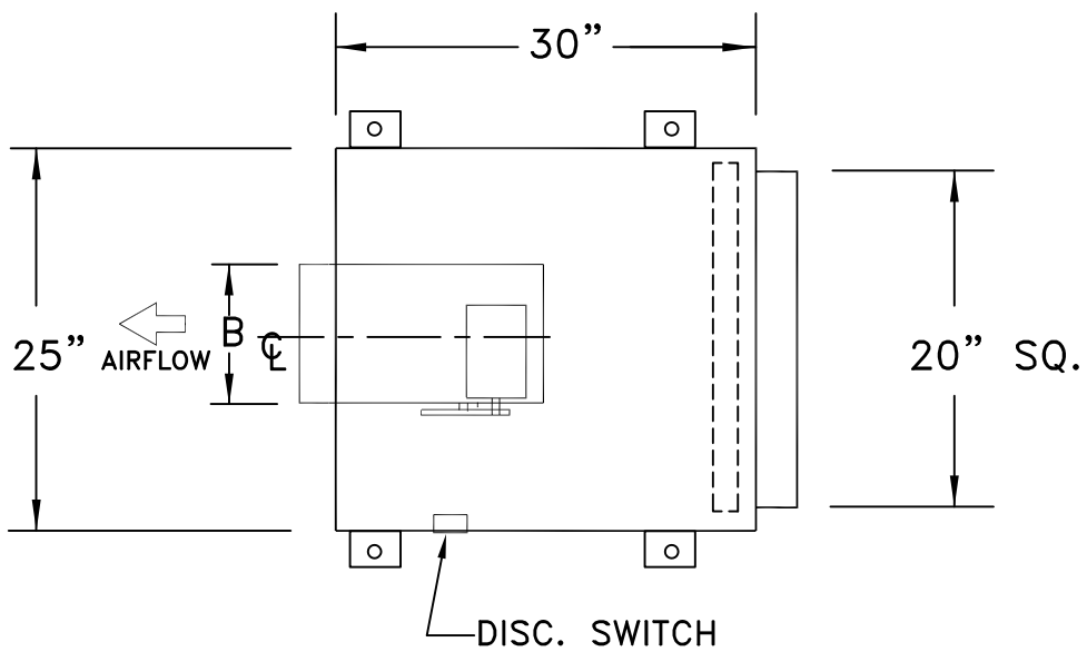
PLAN VIEW
