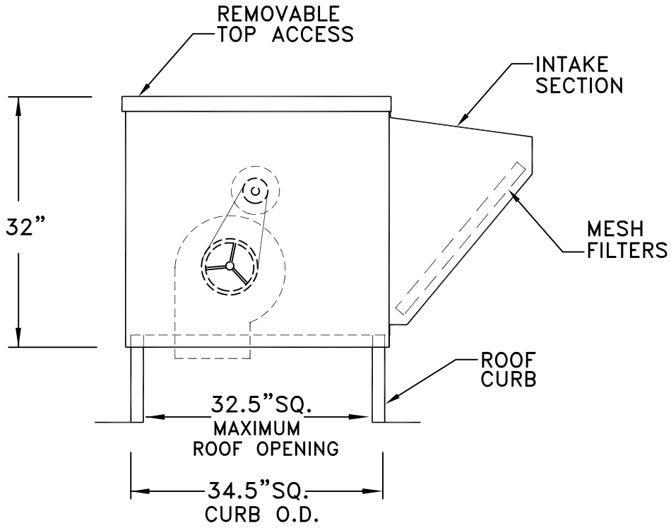
SECTION VIEW
