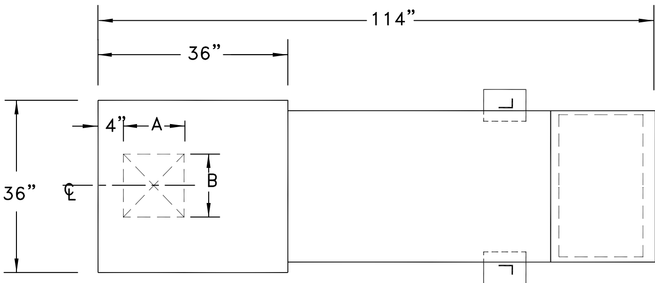
SECTION VIEW
